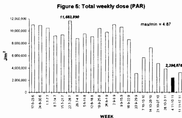
Figure 3–5. Total weekly dose fluctuations for UV-B (Figure 3), UV-A (Figure 4), and PAR (Figure 5). All maximum values (light gray columns) occurred during the period 22–28 July, 1995, while all minima (dark columns) occurred during 4–10 November, 1995. The max/min ratio increases with decreasing wavelength: 8.22 for UV-B; 6.06 for UV-A; and 4.87 for PAR.
