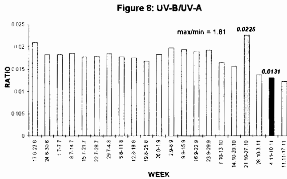
Figure 6–8. Spectral balance of solar UV-B, UV-A and PAR bands. Although total weekly dose was highest in the period 22–28 July 1995, (Figures 3–5), the relative proportion of UV/PAR photons was highest between 5–11 August 1995 (Figures 6 and 7; light gray columns). The minimum values were observed in the period 28 October–3 November, 1995 (Figures 6 and 7; dark columns). In other words, in the fall months, the weekly UV dose declines more rapidly than the weekly PAR dose. The UV-B/UV-A ratio (Figure 8) does not decline as much as the UV-B/PAR and UV-A/PAR ratios.
